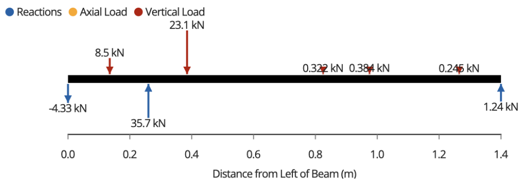
Figure 9 - Force diagram
