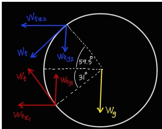
Forces acting in idler gear,
