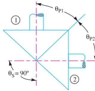
Figure 5 - Mitre gears.
