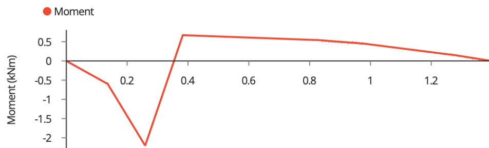
Figure 10 - Bending moment diagram
