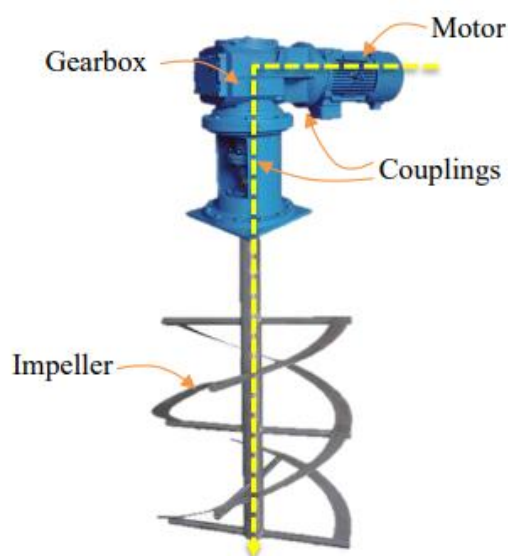
Figure 2 - Basic power flow
