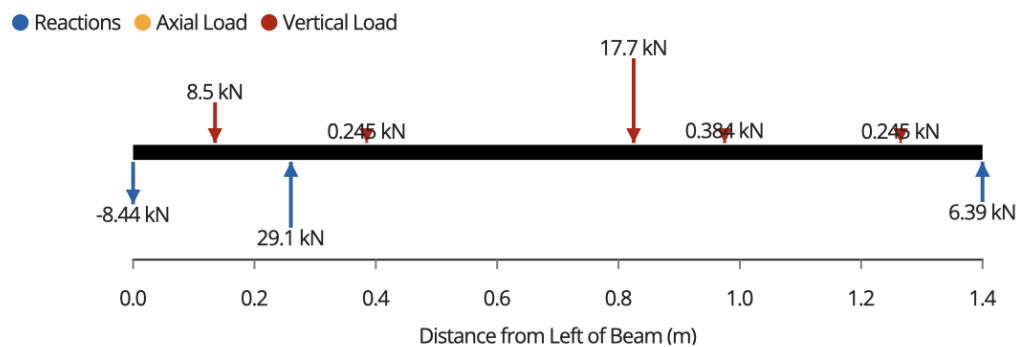
Figure 11 - Force diagram
