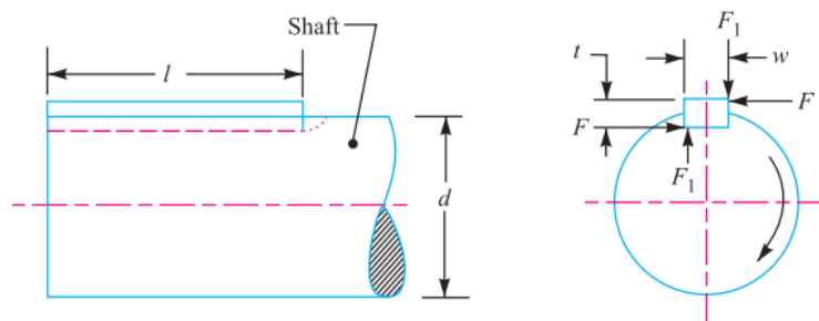
Figure 33 - Forces acting on a sunk key.
