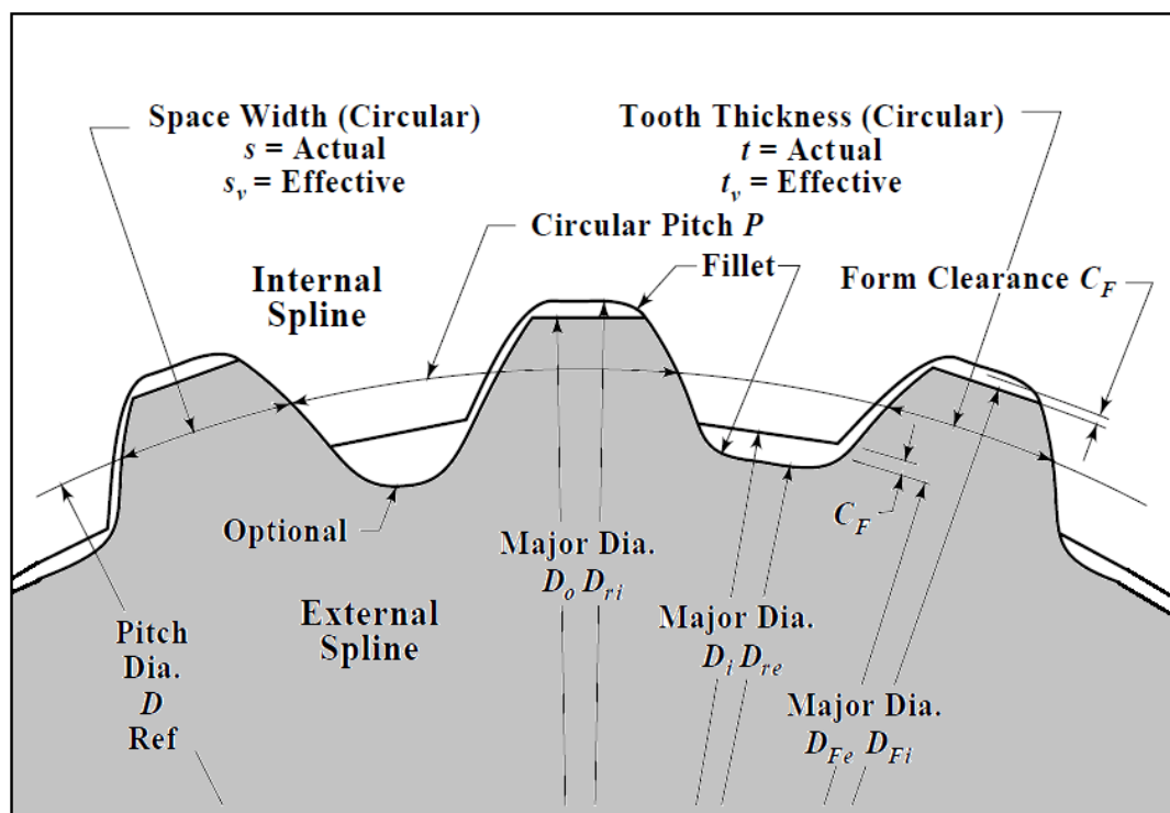
Figure 35 - Splines terminology.
