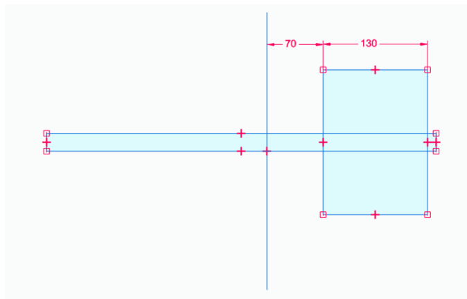
Figure 29-Input shaft configuration
