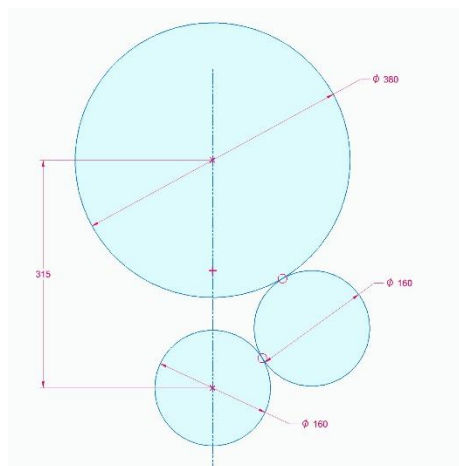
Figure 4 - Reverse gear.
