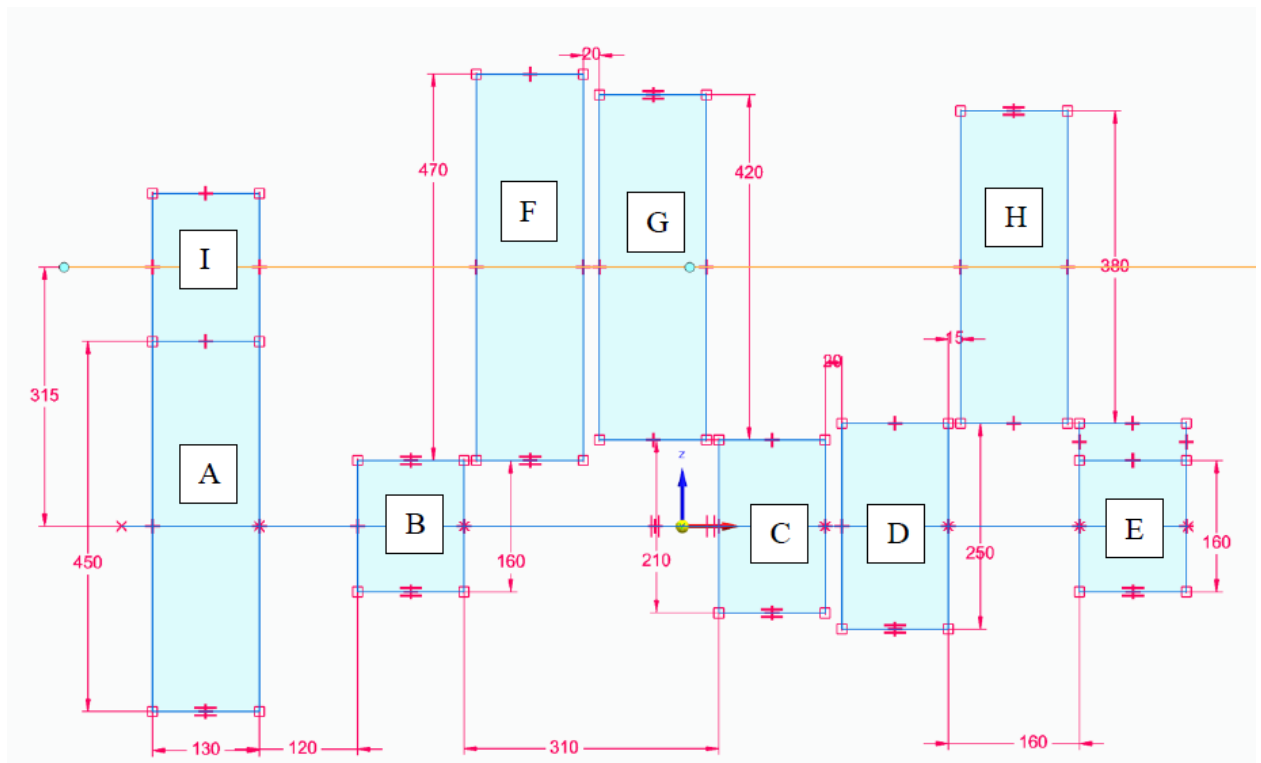
Figure 3 : Gear box layout
