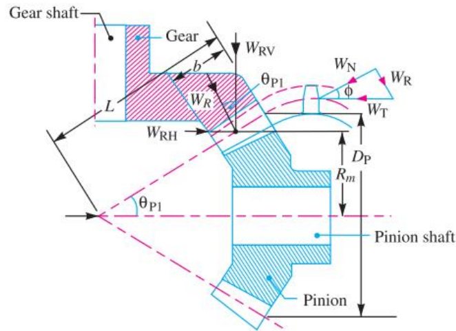
Figure 6 - Forces acting on a bevel gear.
