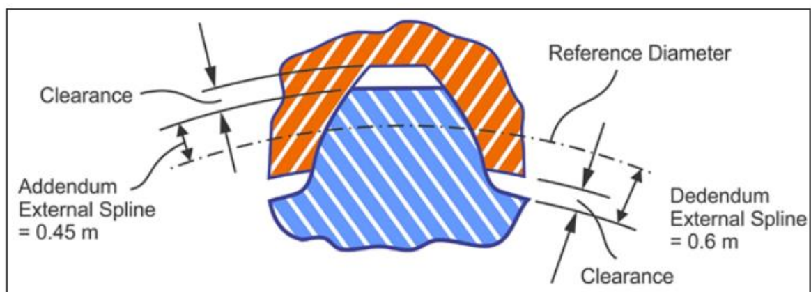
Figure 36 - Flank centred spline connection
