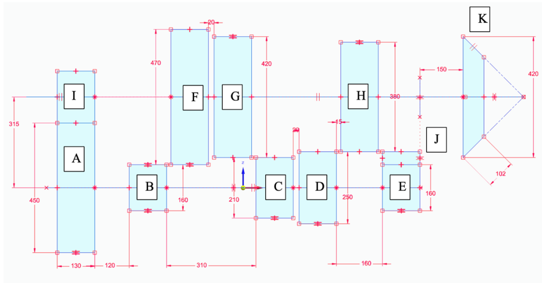
Figure 42 – Gearbox configuration
